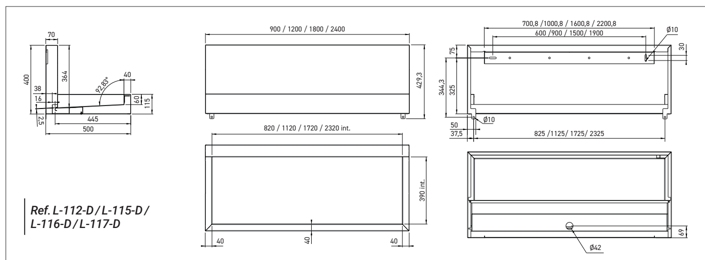
Integrated faucets RONDEO soap & water & air
