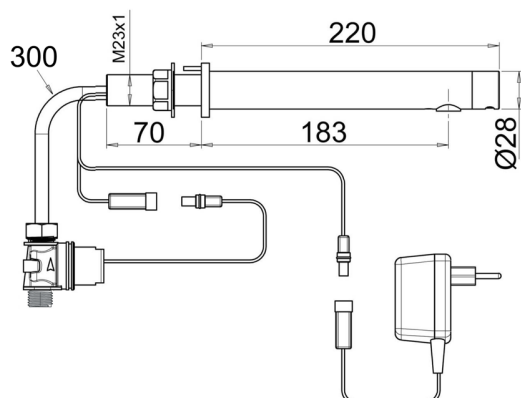
RES-141-S1 pannel mounted, transformer
