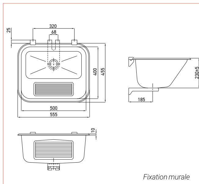
Fixation murale
